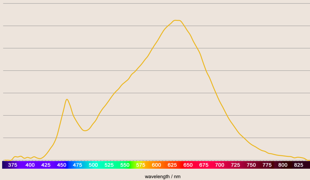
SPECTRAL POWER DISTRIBUTION OF LEDON 8.5W A60
